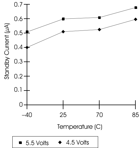
Graph 2-3: Standby Current ( I_{SB} )
