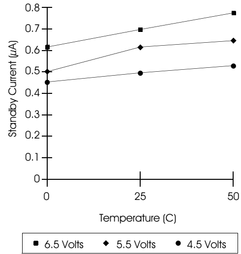
Graph 2-7: Standby Current ( I_{SB} )
