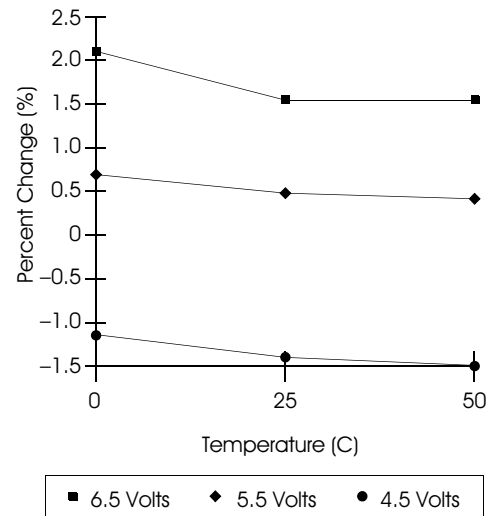
Graph 2-8: Oscillator Stability
