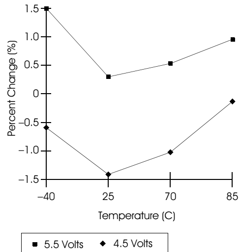
Graph 2-4: Oscillator Stability
