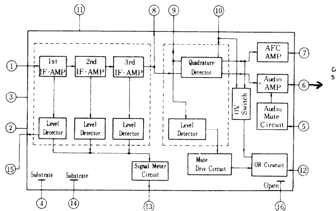
HA-1137 BLOCK DIAGRAM
