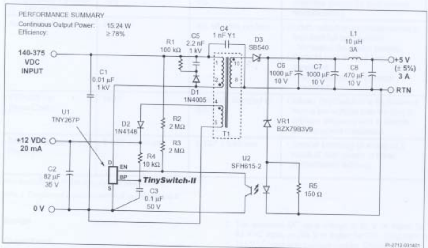
Figure 16. 15 W PC Standby Supply.
