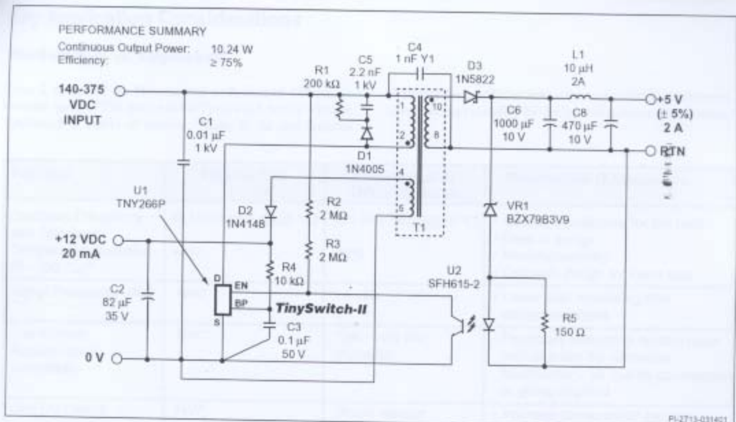
Figure 15. 10 W PC Standby Supply.
