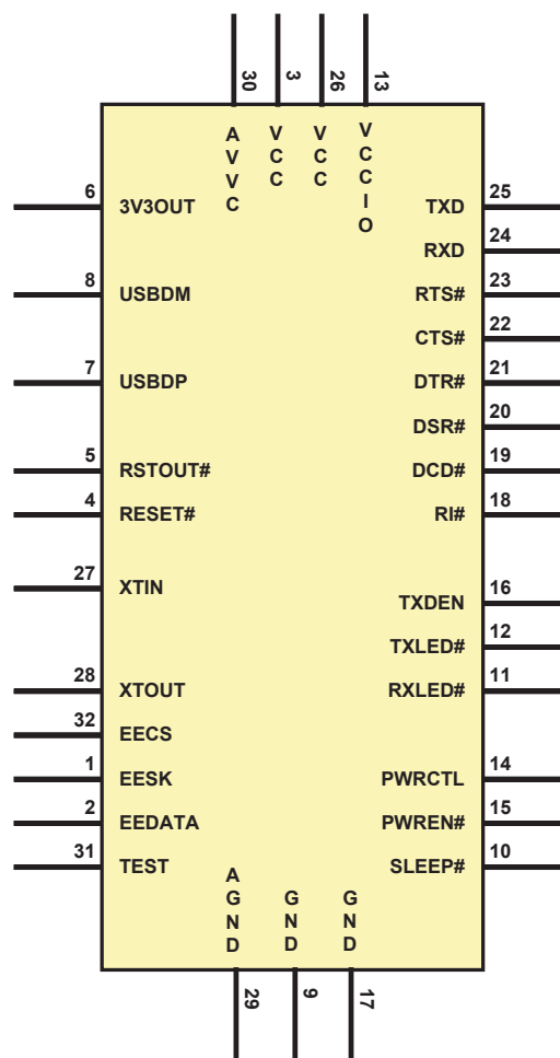
Figure 2 Pin-Out (Schematic Symbol )
