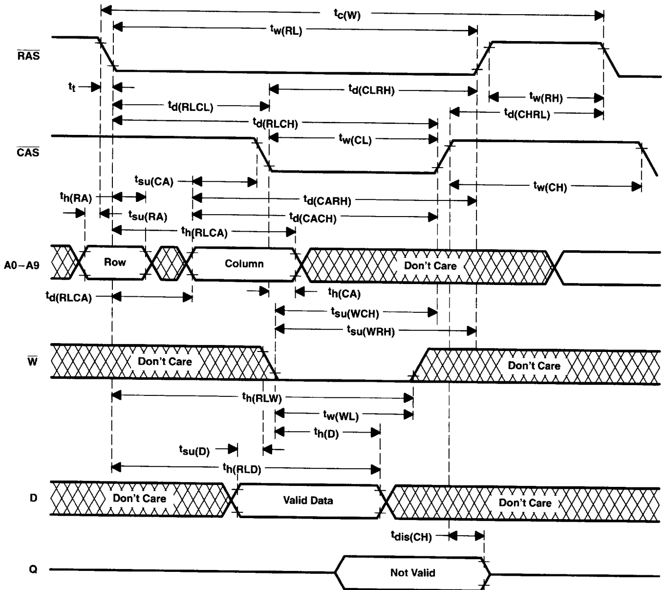
Figure 4. Write-Cycle Timing
