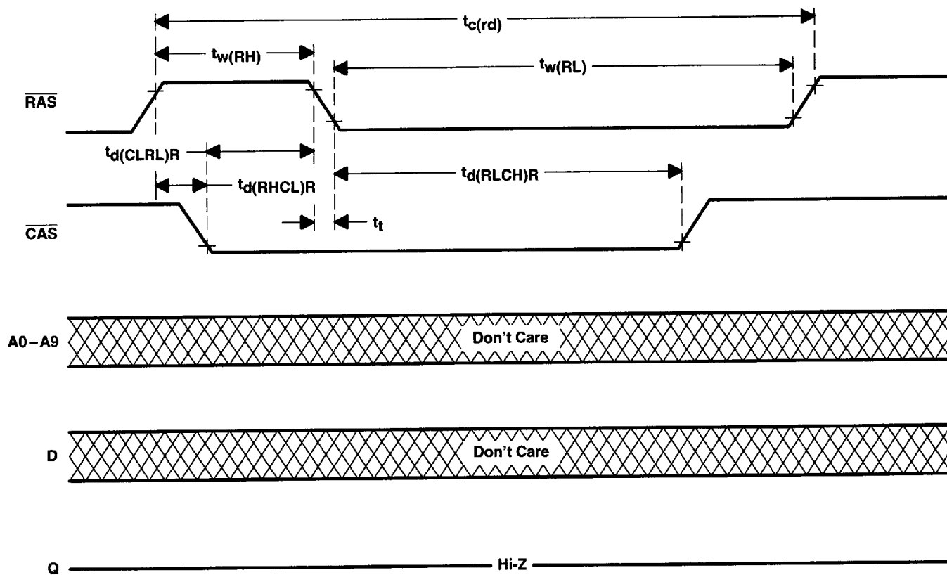
Figure 11. Automatic-CBR-Refresh-Cycle Timing
