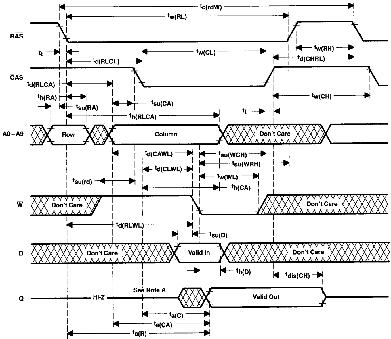
Figure 5. Read-Write/Read-Modify-Write-Cycle Timing
