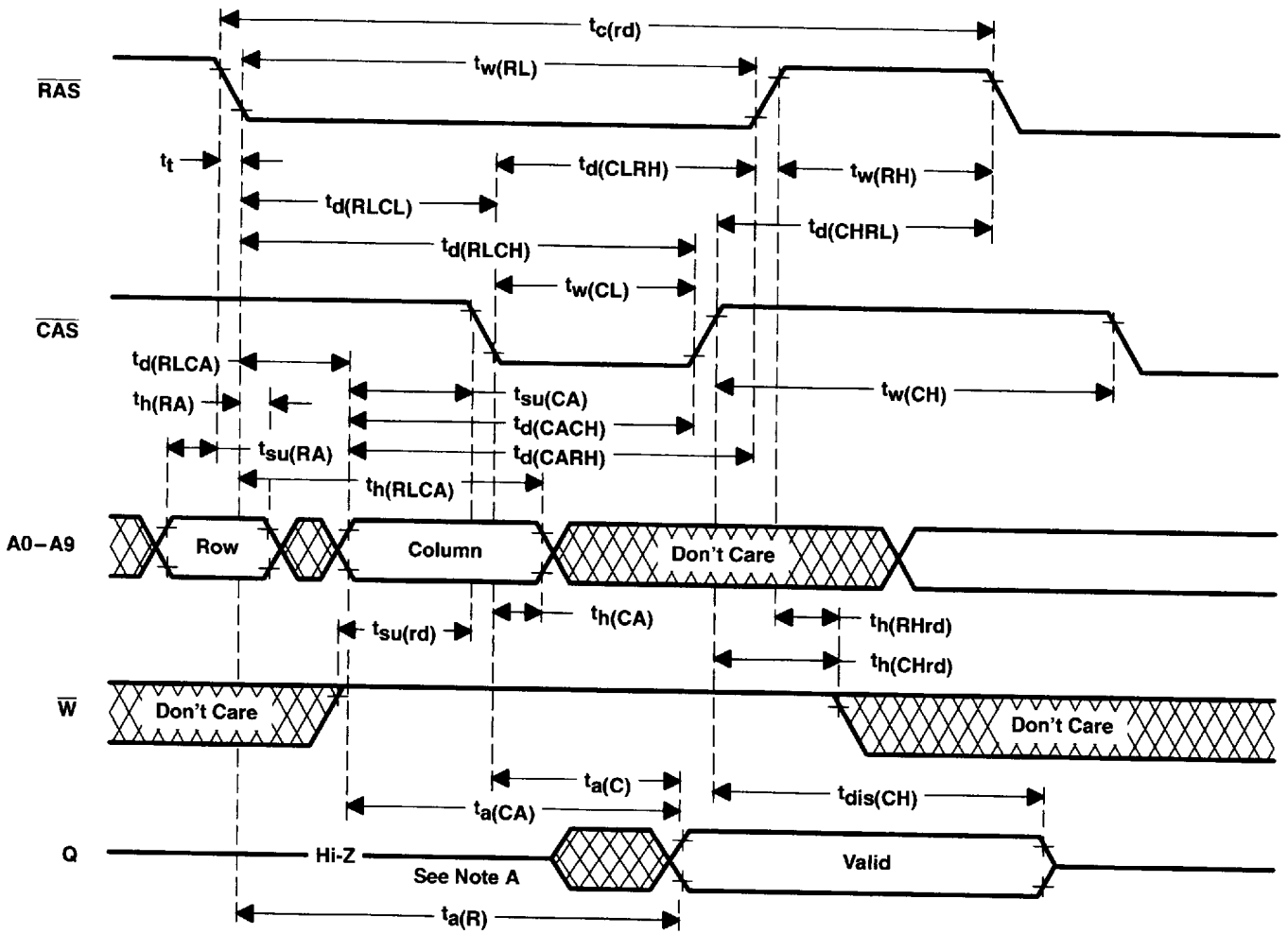
Figure 2. Read-Cycle Timing
