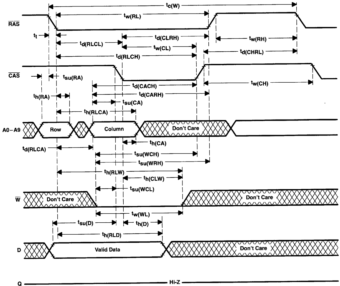
Figure 3. Early-Write-Cycle Timing
