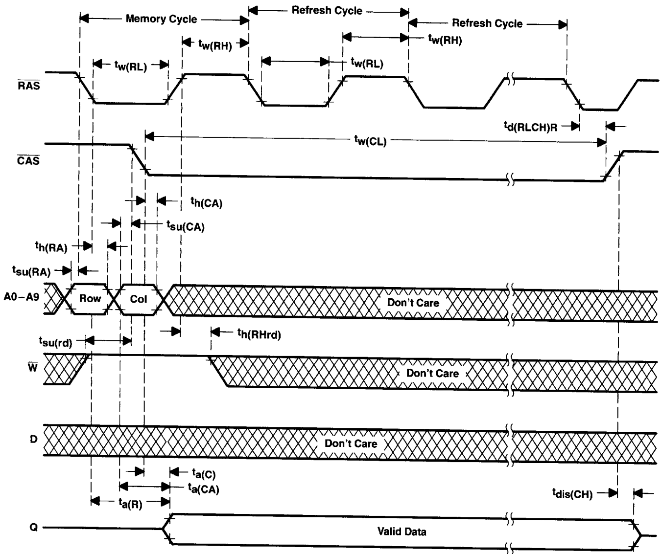
Figure 10. Hidden-Refresh-Cycle Timing
