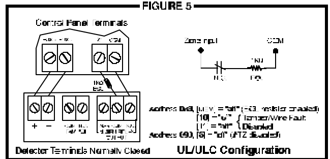
N.C. Contacts, With EOL Resistor (UL/ULC)
