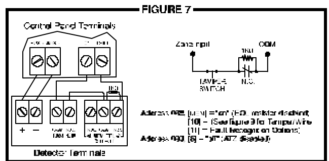
N.C. Contacts, Without EOL Resistor, With Tamper Recognition
